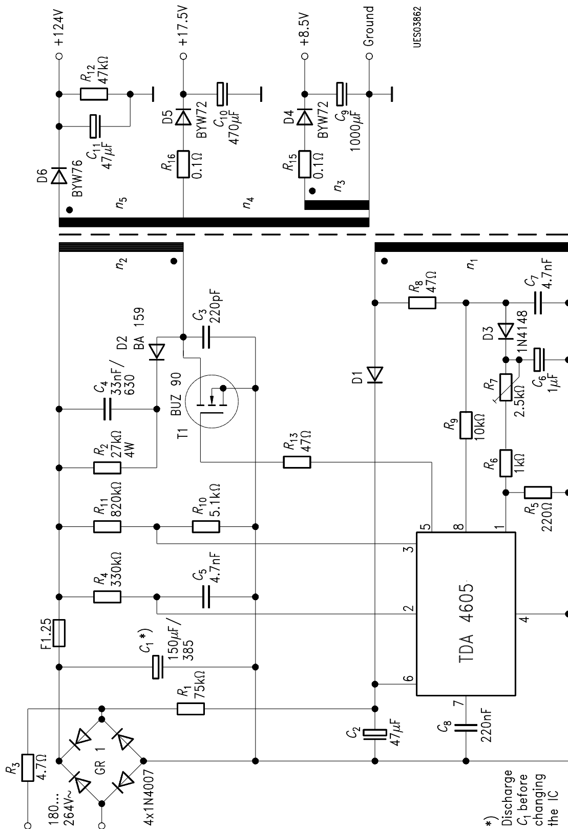
Application Circuit
