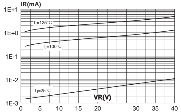
Fig. 8-2: Reverse leakage current versus reverse voltage applied (typical values) (1N5819).
