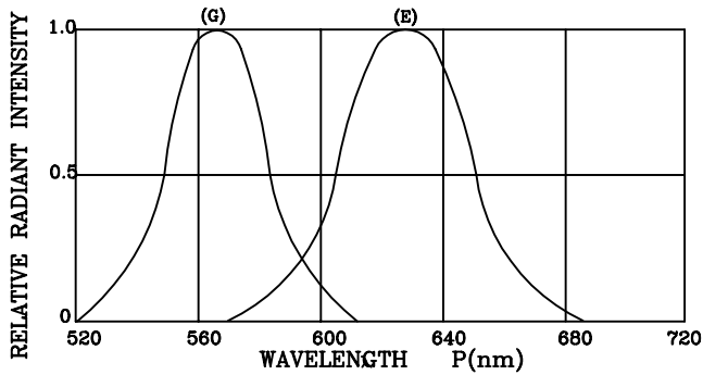
SPECTRAL DISTRIBUTION
