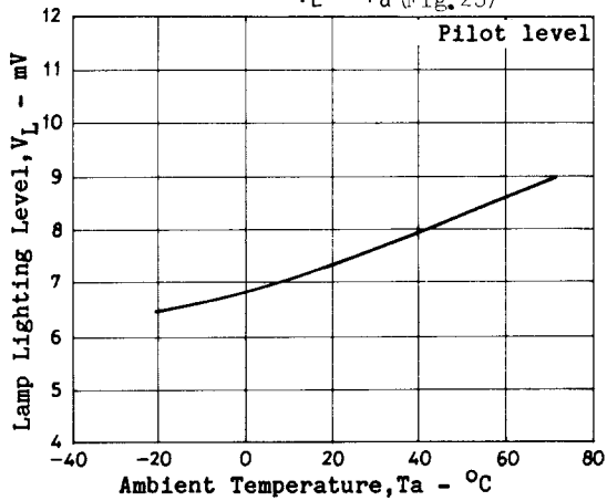
Lamp Lighting Level, V_L - T_a (Fig. 25)
