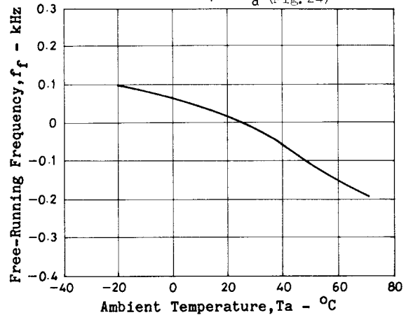
Free-Running Frequency, f_f - T_a (Fig. 24)
