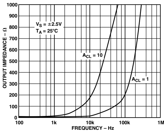
TPC 21. Output Impedance vs. Frequency
