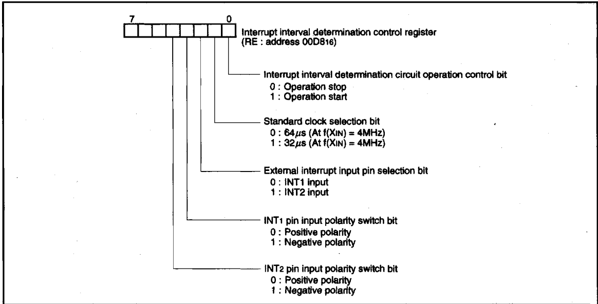
Fig. 42 Structure of interrupt space distinguish control register
