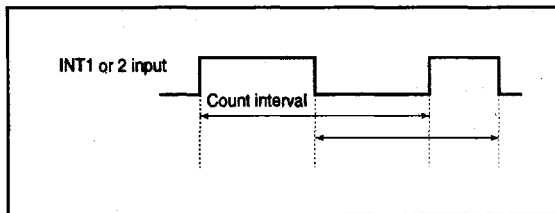
Fig. 43 Measuring interval
