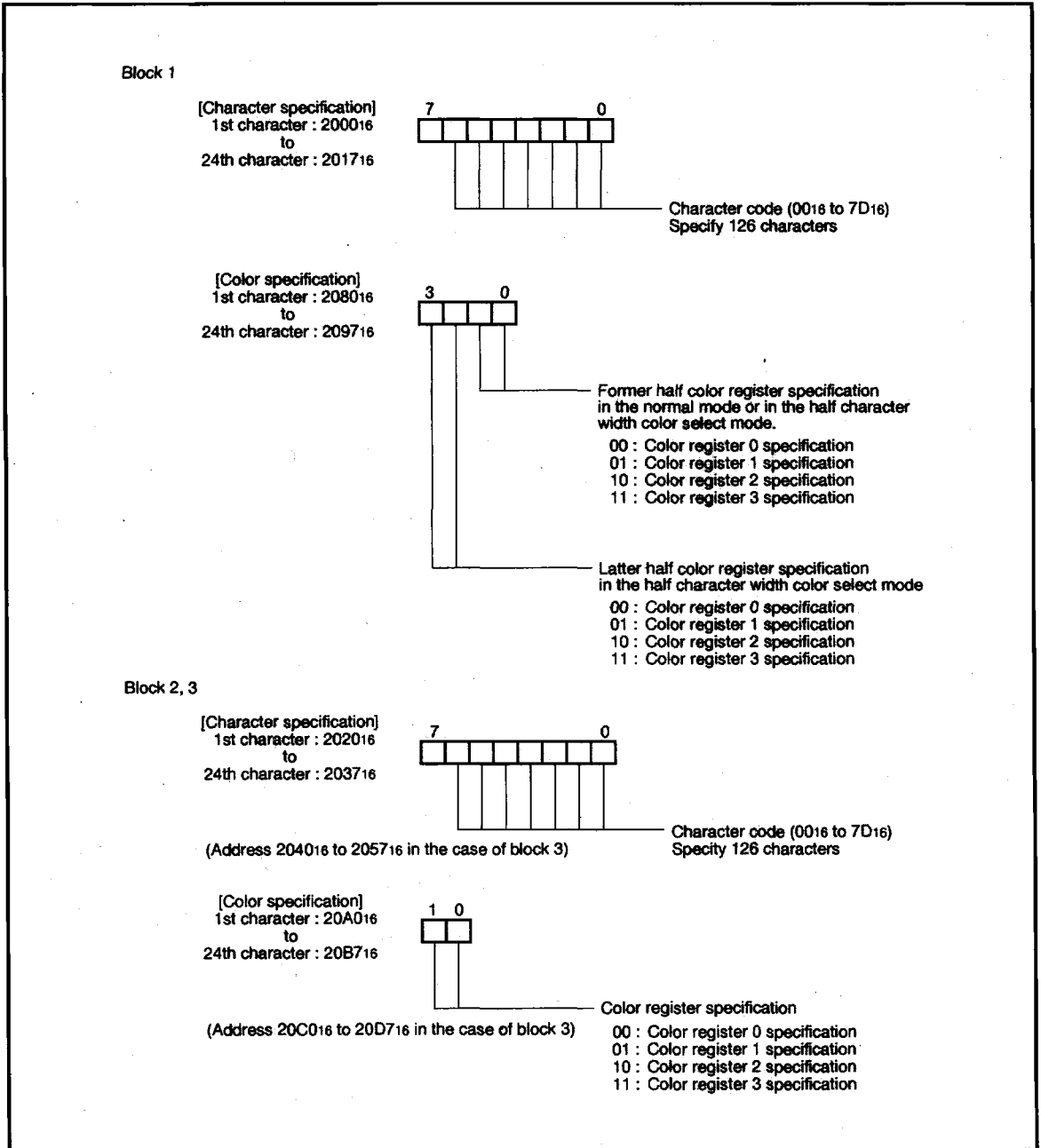
Fig. 31 Structure of the CRT display RAM
