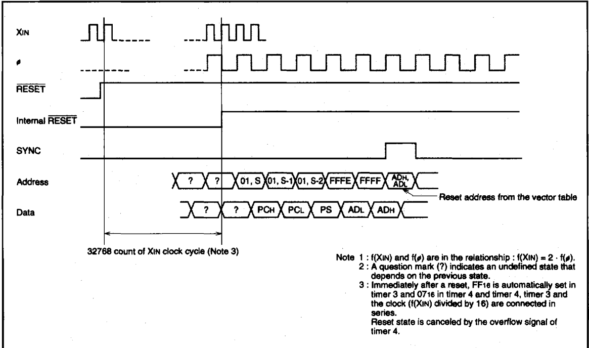
Fig. 46 Reset sequence
