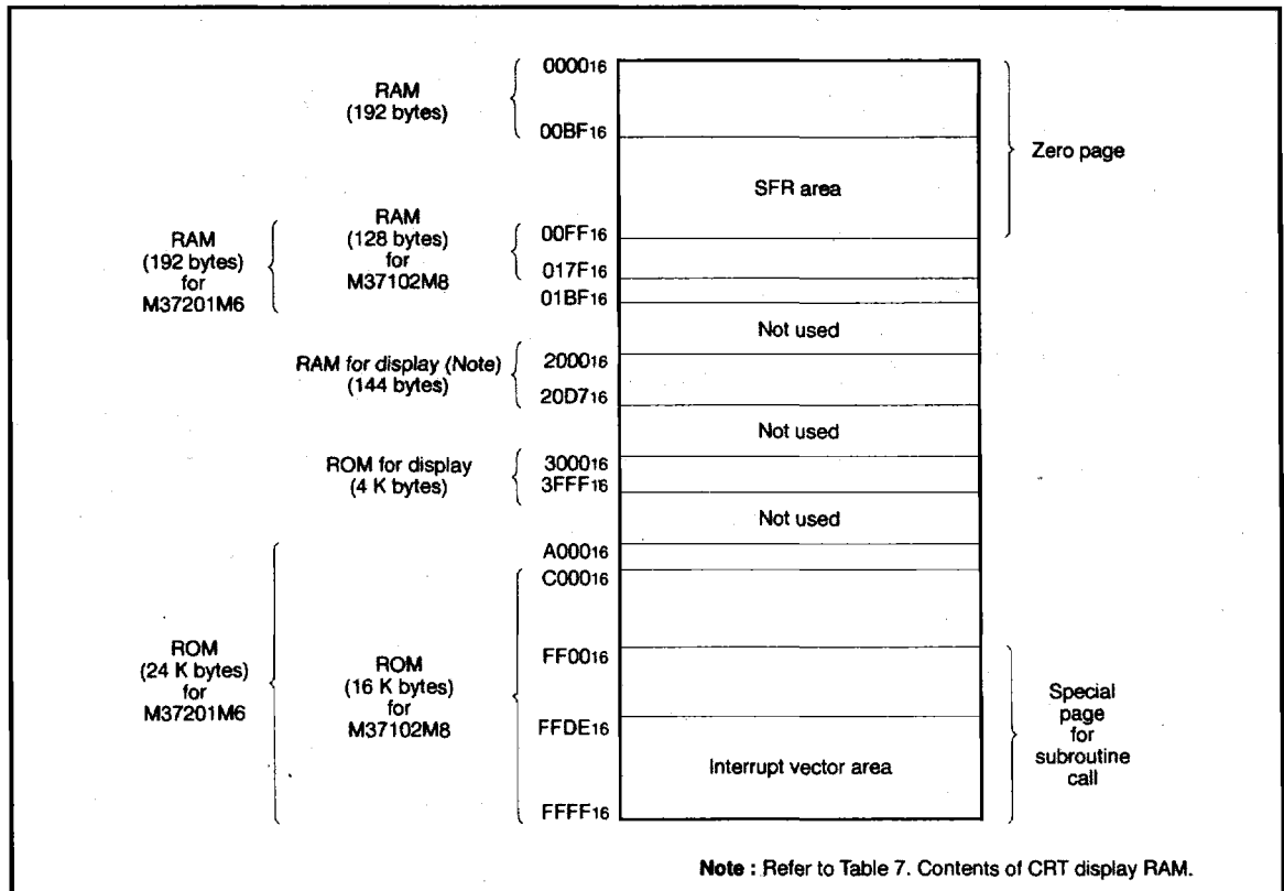
Fig. 2 Memory map
