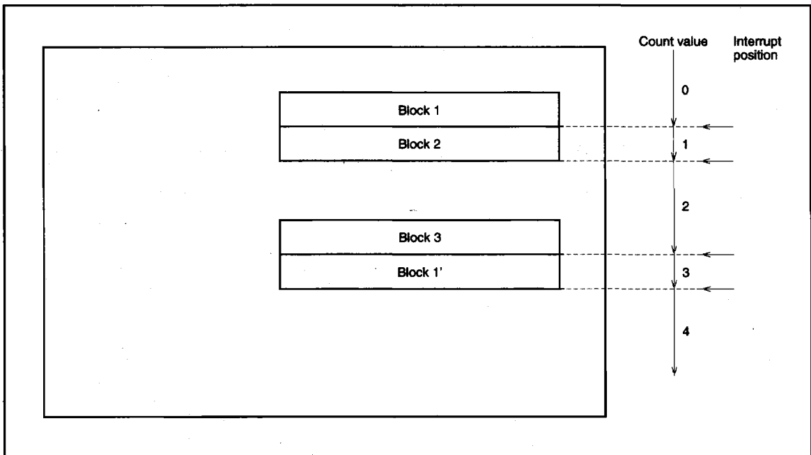
Fig. 35 Timing of CRT interrupt and count value of display block counter
