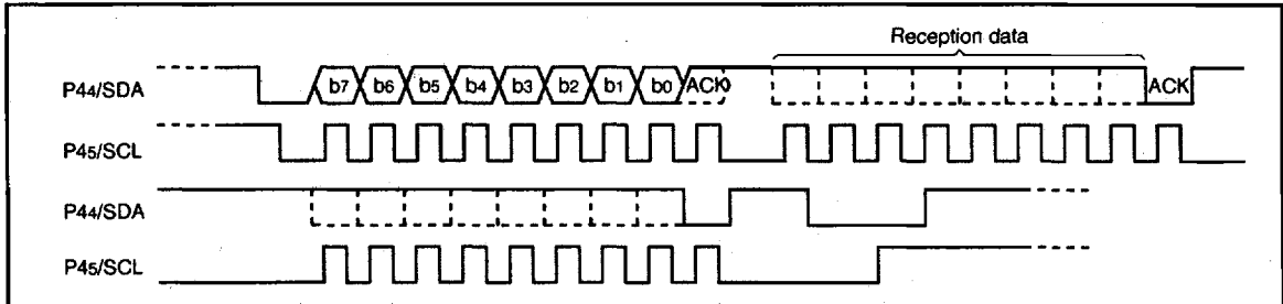
Fig. 14 Master reception timing
