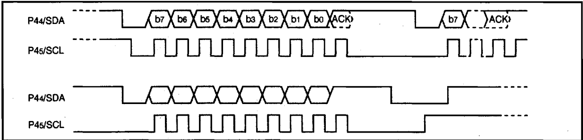
Fig. 13 Master transmission timing
