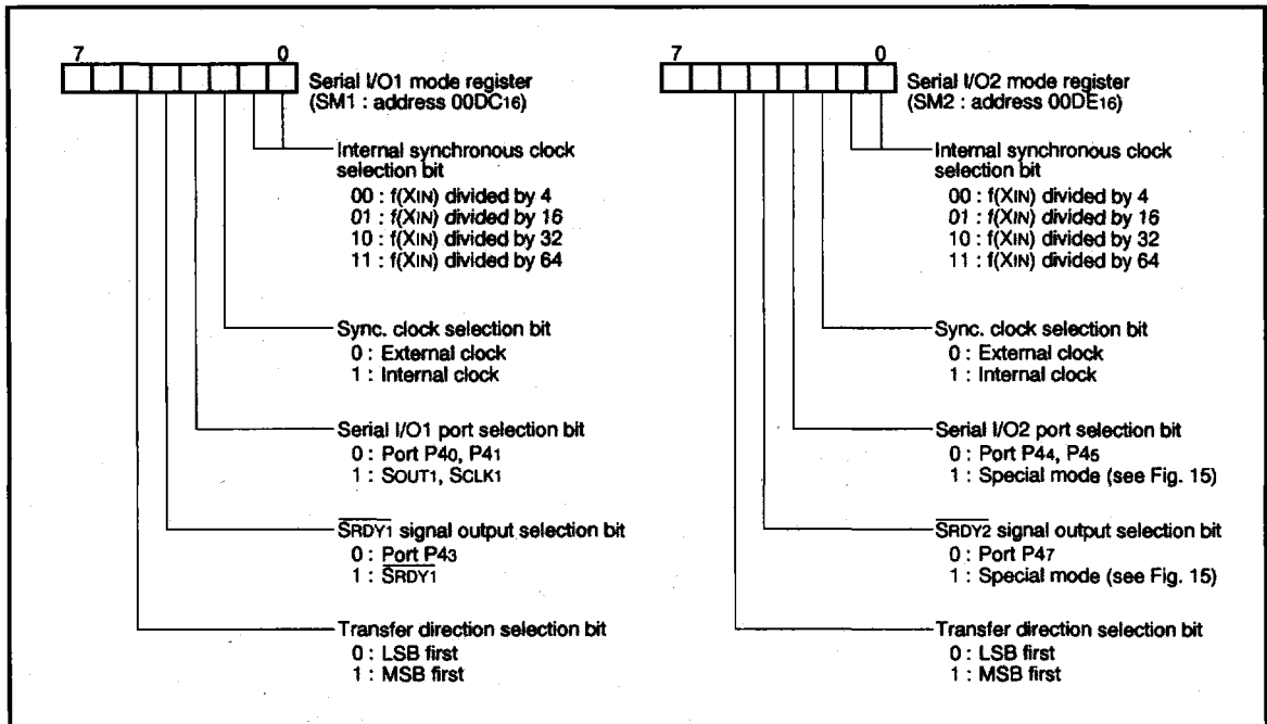
Fig. 11 Structure of serial I/O i mode register
