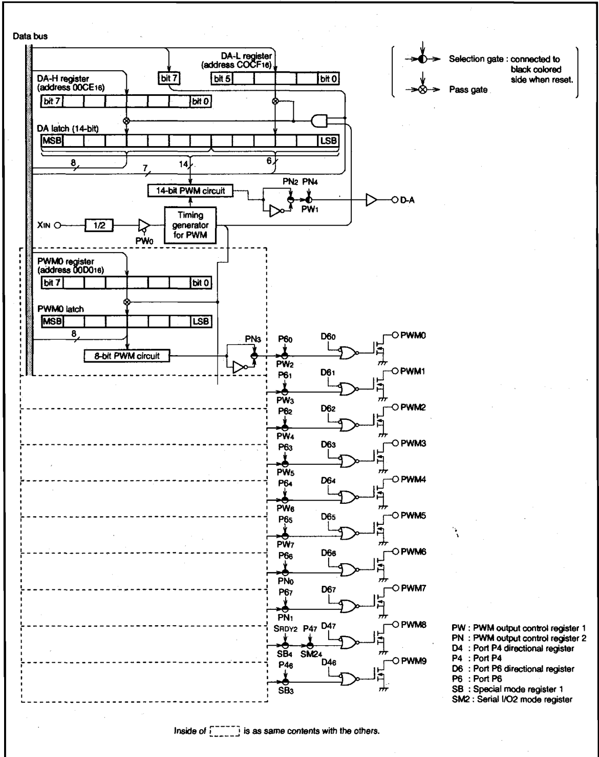
Fig. 16 PWM block diagram
