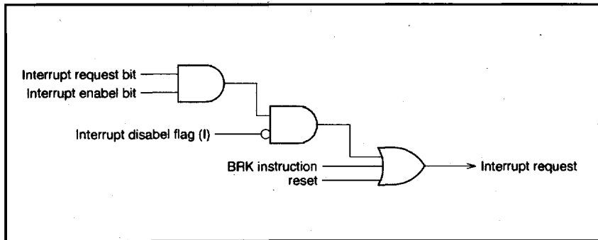
Fig. 5 Interrupt control
