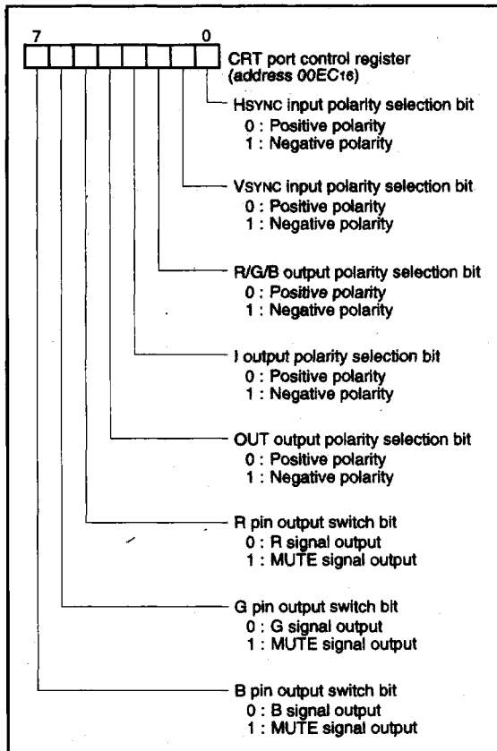
Fig. 39 Structure of CRT port control register
