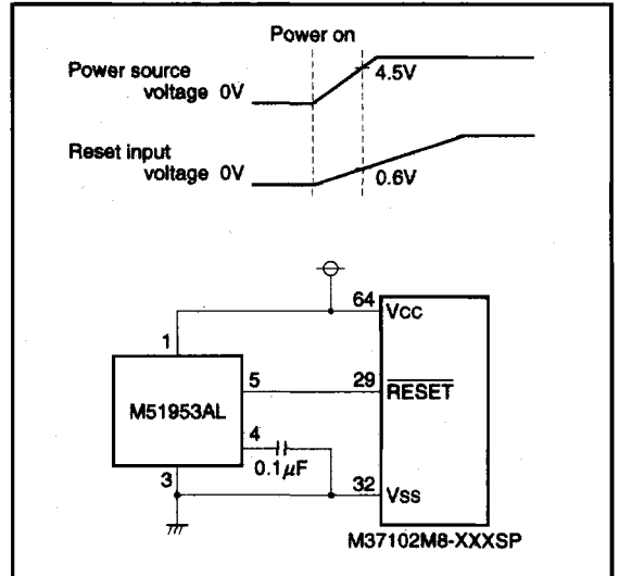
Fig. 45 Example of reset circuit
