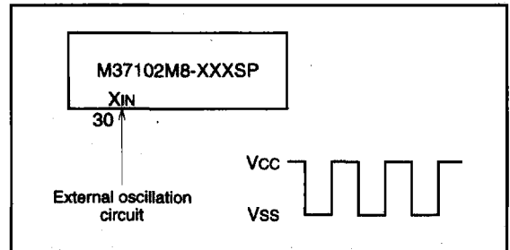
Fig. 49 External clock input circuit example
