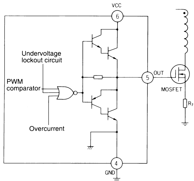
Fig. 19 Output circuit
