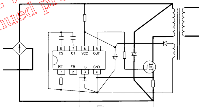
Fig. 27 Vcc line and ground line (2) for FA5314/15
