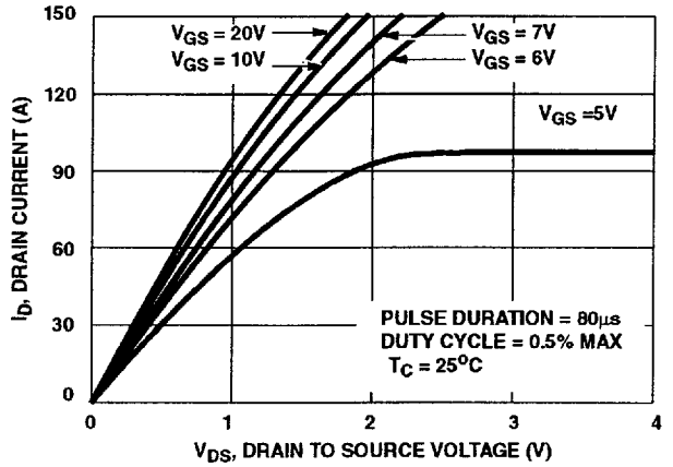
FIGURE 8. SATURATION CHARACTERISTICS
