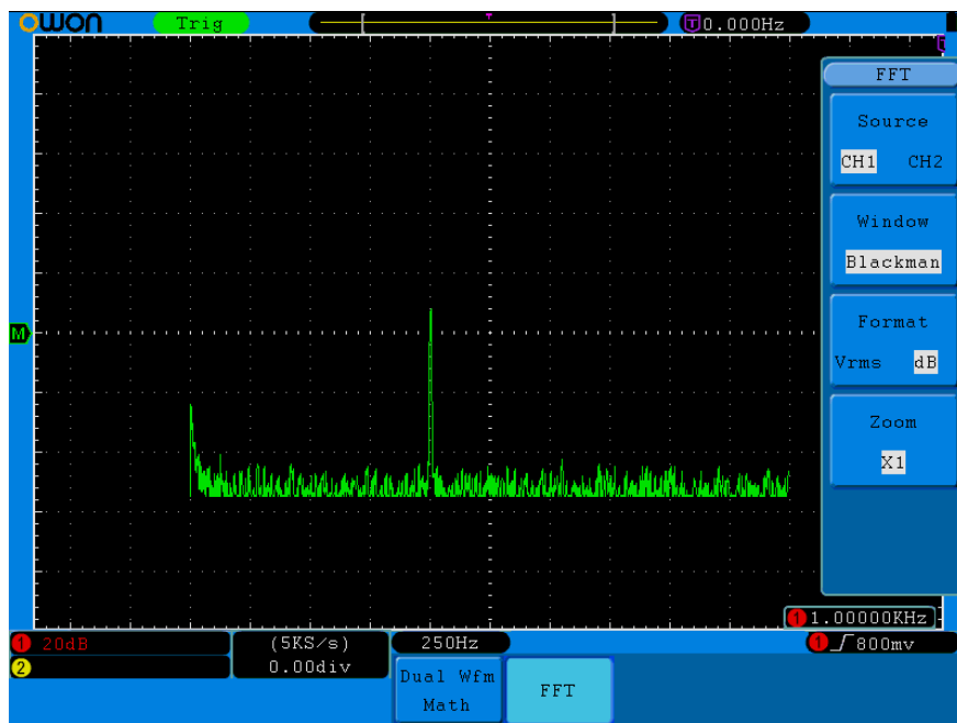
Fig.5-11. Blackman window
