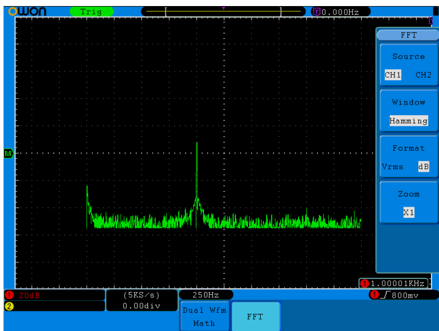
Fig.5-9 Hamming window
