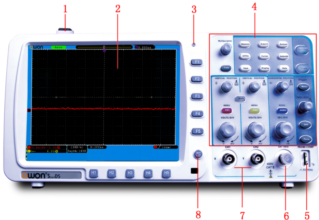
Fig. 4-1 Front panel
