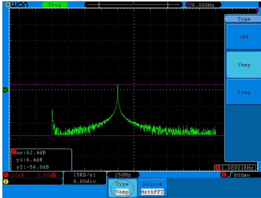
Fig.5-61 wave of Vamp cursor measurement
