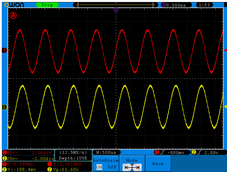
Fig.5-64 Autoscale Horizontal-Vertical multi-period waveforms
