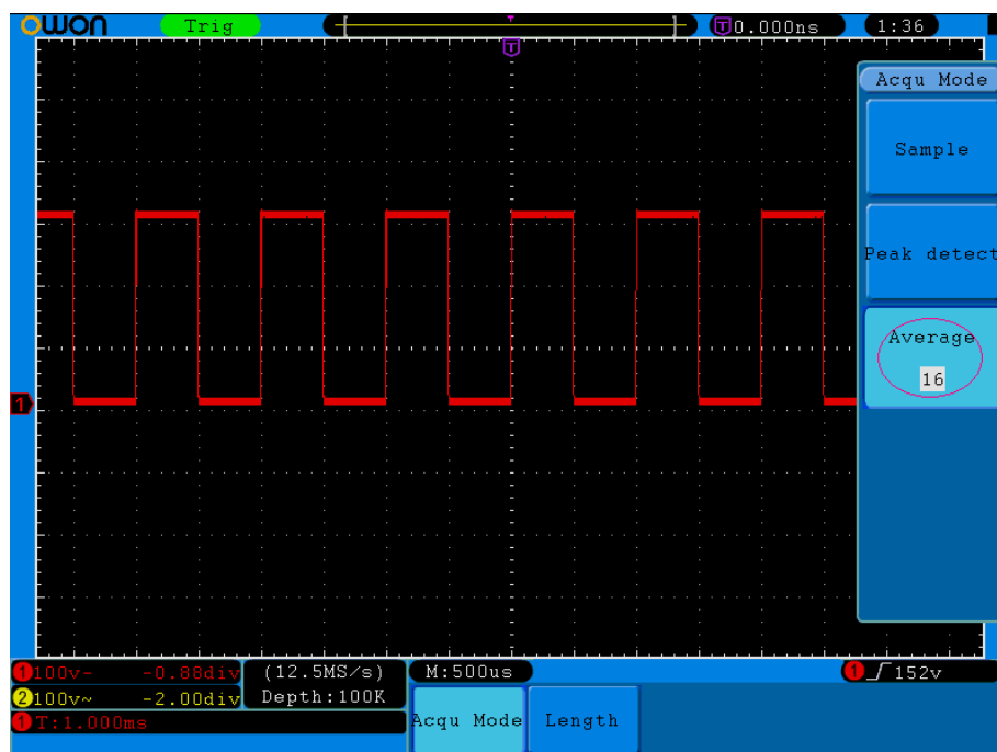
Fig.6-5 Reduce Noise level by using Average function
