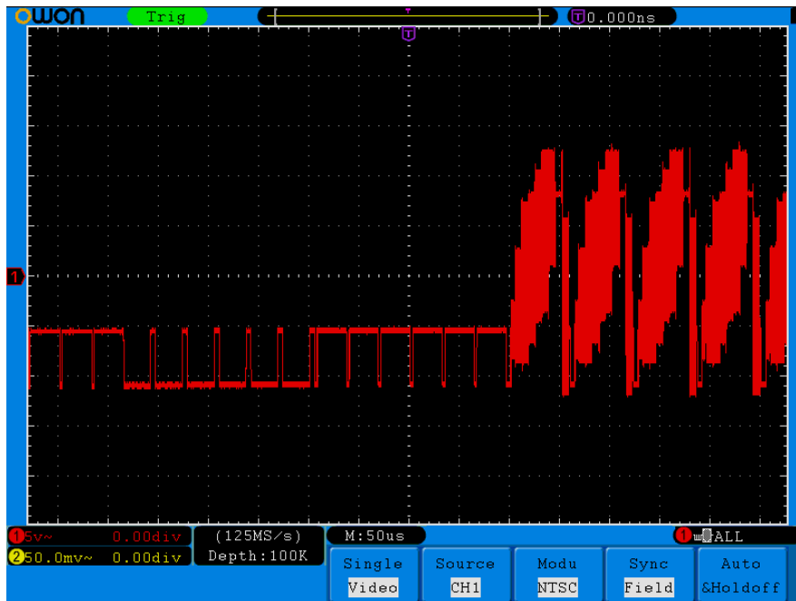
Fig.6-7 Waveform Captured from Video Field Trigger
