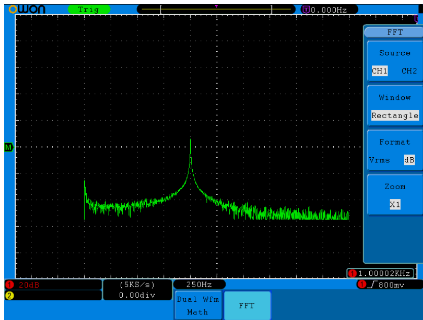
Fig.5-8. Rectangle window
