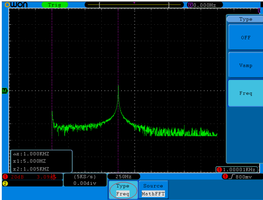
Fig.5-62 wave of Freq cursor measurement
