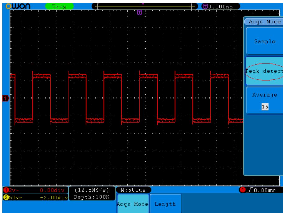
Fig.6-4 Signal with Noises
