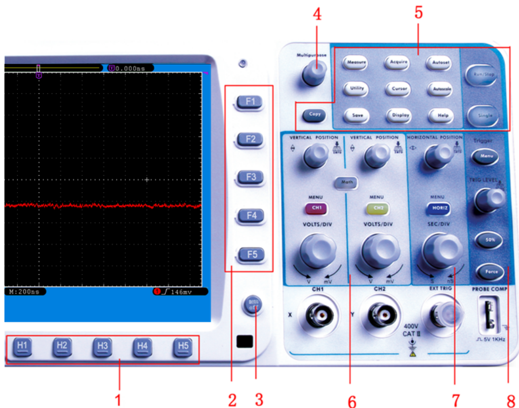
Fig. 4-5 Keys Overview
