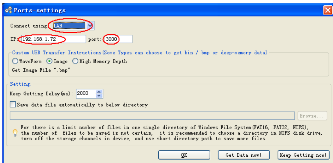
Fig.5-51 Set the network parameters of the OWON Oscilloscope Software
